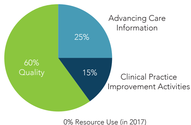
2017 MIPS Scoring
